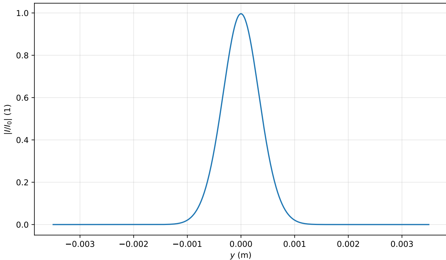
Intensity profile I(x=0, y, z=0.557)/I_0 , P_{in}=0.3P_{cr} , artificial time
